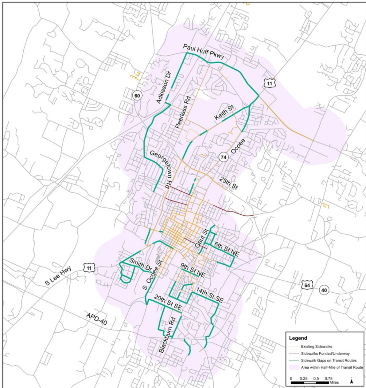
Figure 4.36: Gaps in Pedestrian Network along Existing Fixed-Route Transit
