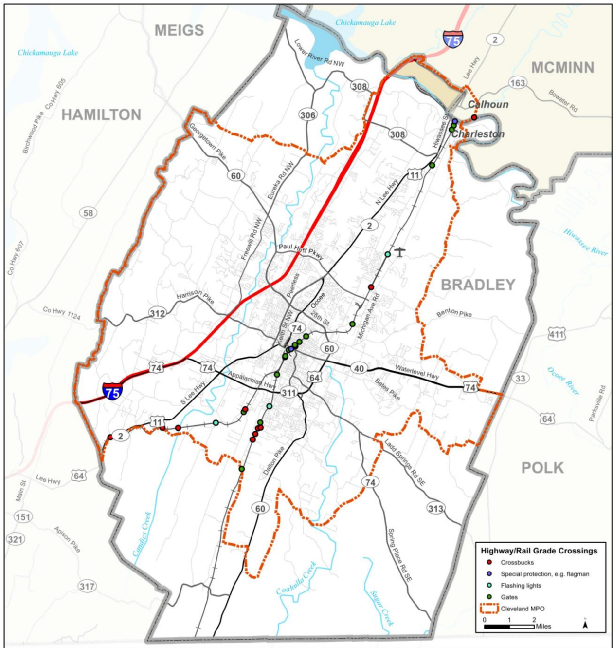
Figure 4.15: Highway/Rail Grade Crossings and Type of Warning Device
