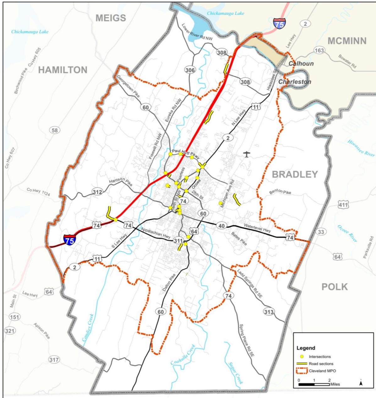
Figure 4.8: High-Crash Locations (Intersections and Road Segments)
