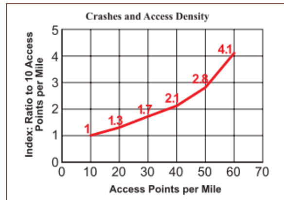
Figure 4.9: Relationship between a road's crash rate and the number of access points per mile. From the Transportation Research Board's Access Management Manual (2003).
