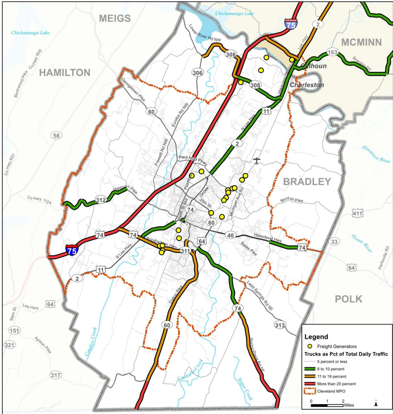
Figure 4.17: Routes with a High Percentage of Truck Traffic
