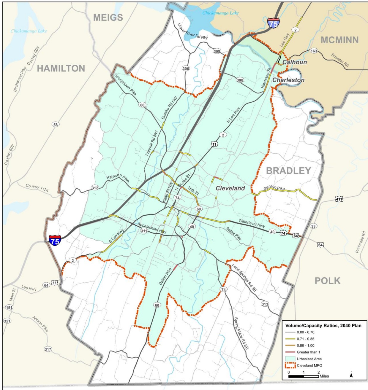
Figure 4.7: Projected Traffic Conditions on Area Roadways With Implementation of the 2040 RTP
